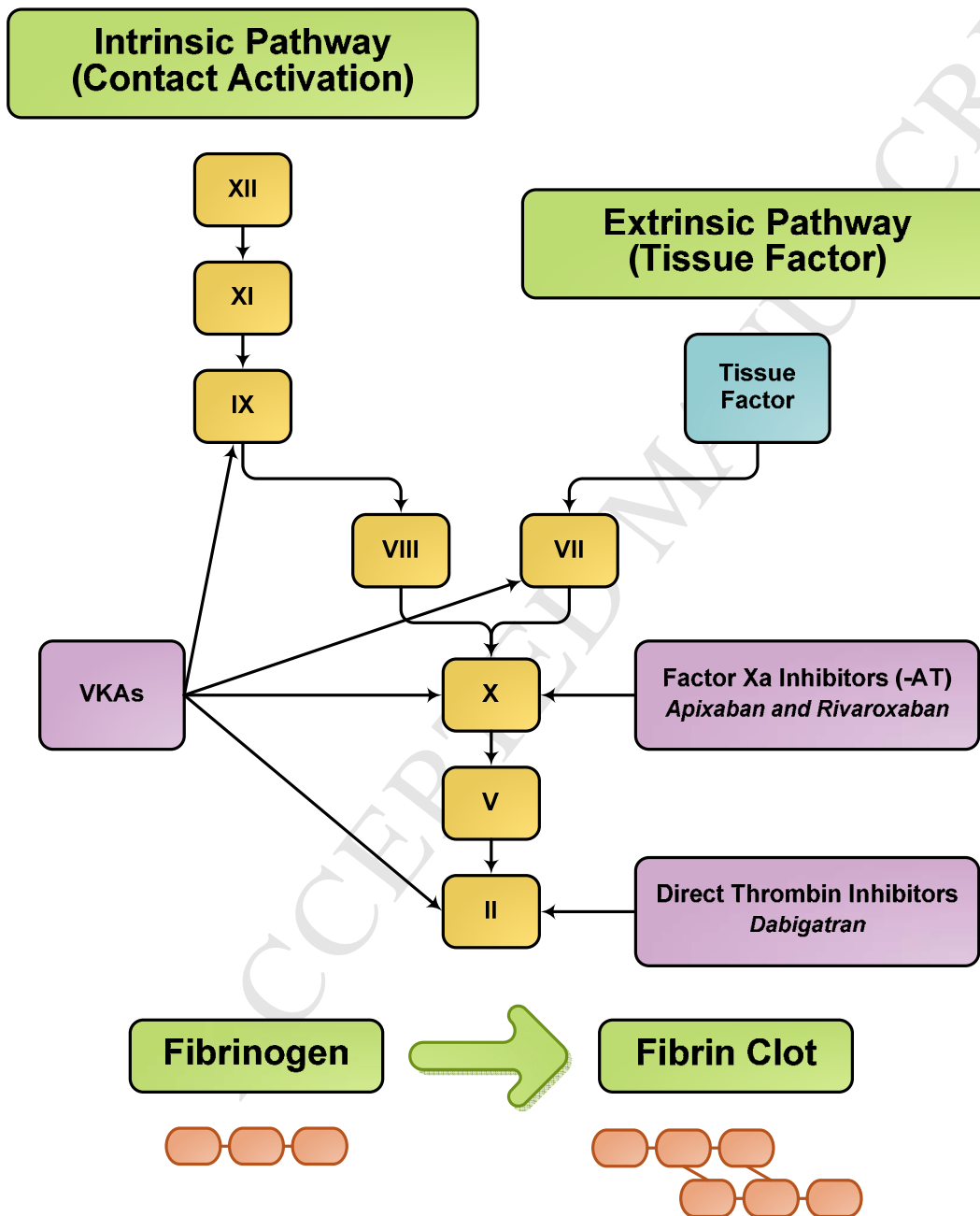
Figure 4. Coagulation Cascade
